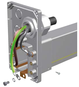
EB40 (open)
