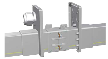
RN-LH (mounted)
